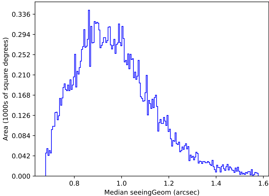
weather_cloudso36v3.4_10yrs Yr 1 u band: Median seeingGeom
