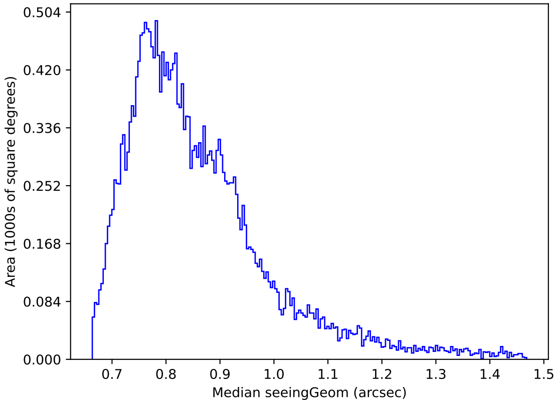
weather_cloudso36v3.4_10yrs Yr 1 r band: Median seeingGeom
