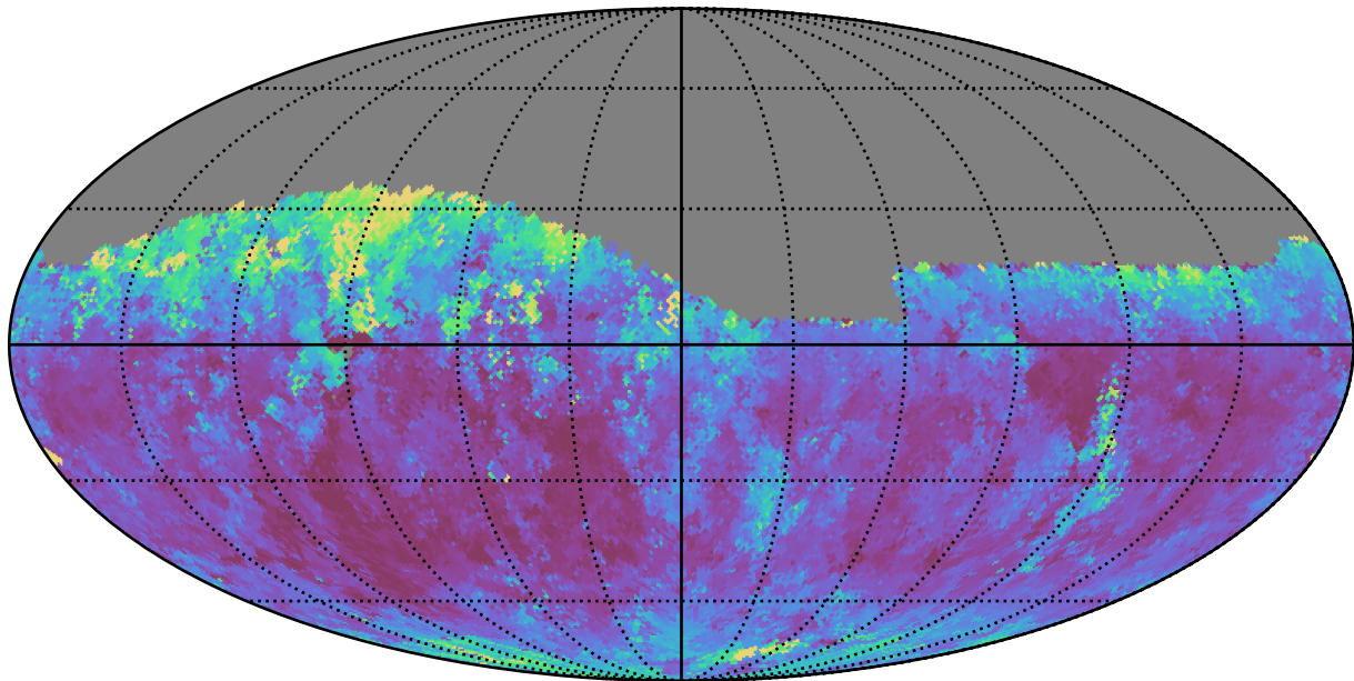
weather_cloudso36v3.4_10yrs Yr 1 i band: Median seeingGeom
