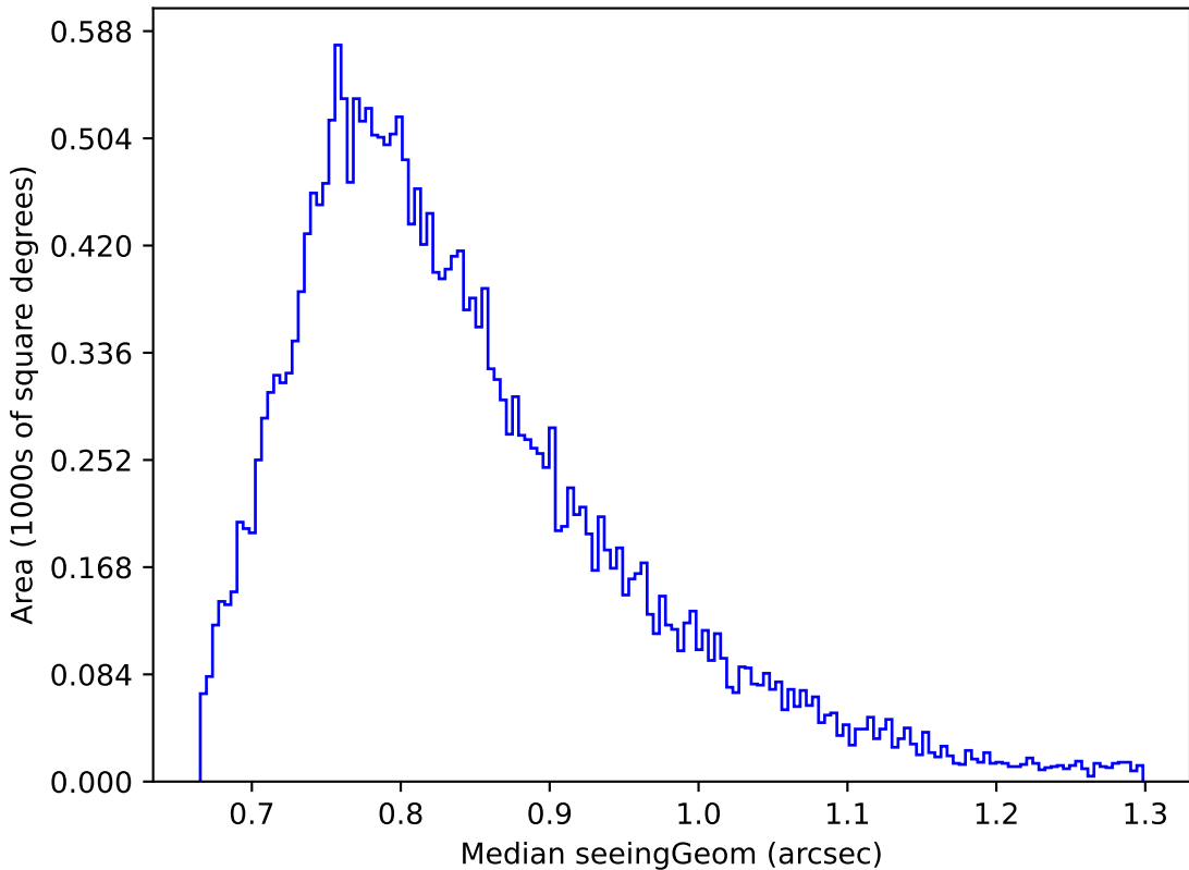
weather_cloudso36v3.4_10yrs Yr 1 i band: Median seeingGeom
