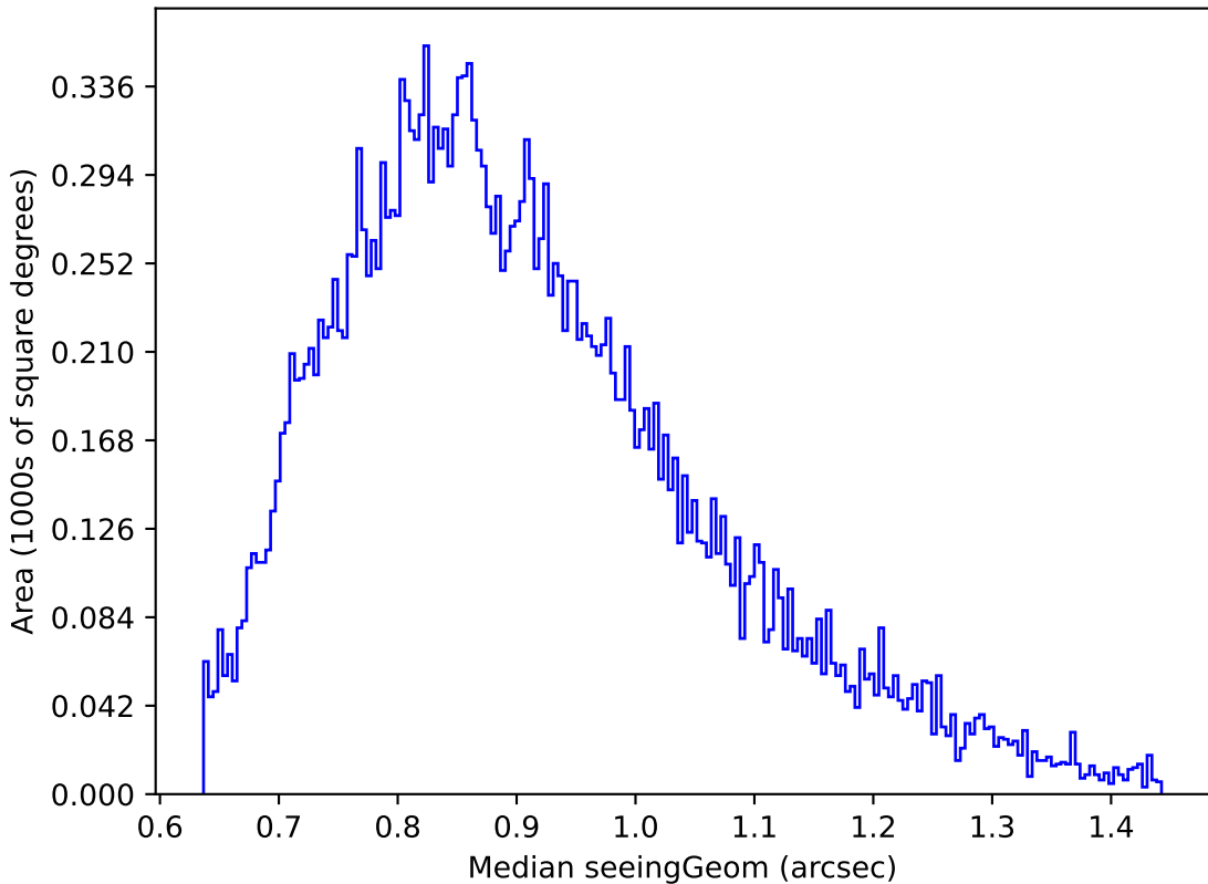
weather_cloudso36v3.4_10yrs Yr 1 g band: Median seeingGeom
