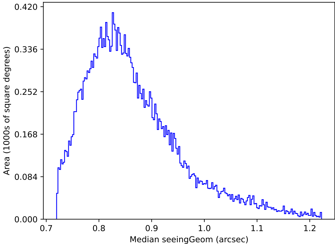
weather_cloudso36v3.4_10yrs Yr 1 all bands: Median seeingGeom
