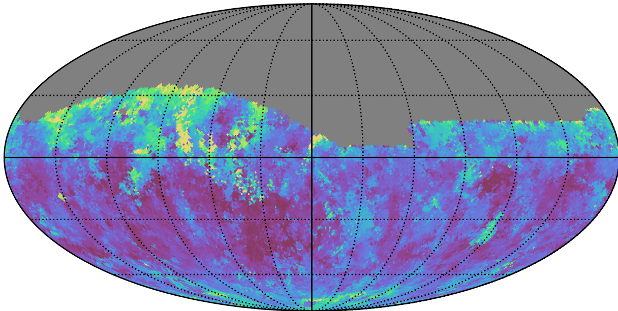
weather_cloudso36v3.4_10yrs Yr 1 z band: Median seeingEff
