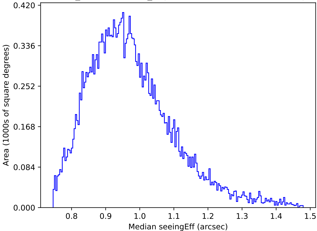
weather_cloudso36v3.4_10yrs Yr 1 z band: Median seeingEff
