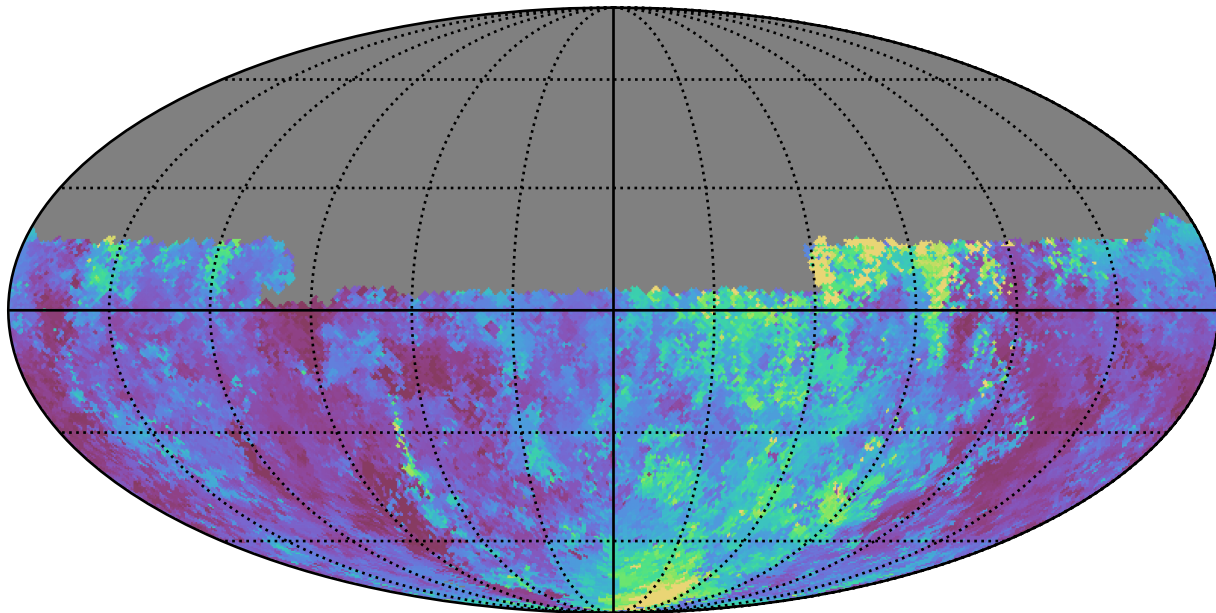
weather_cloudso36v3.4_10yrs Yr 1 u band: Median seeingEff
