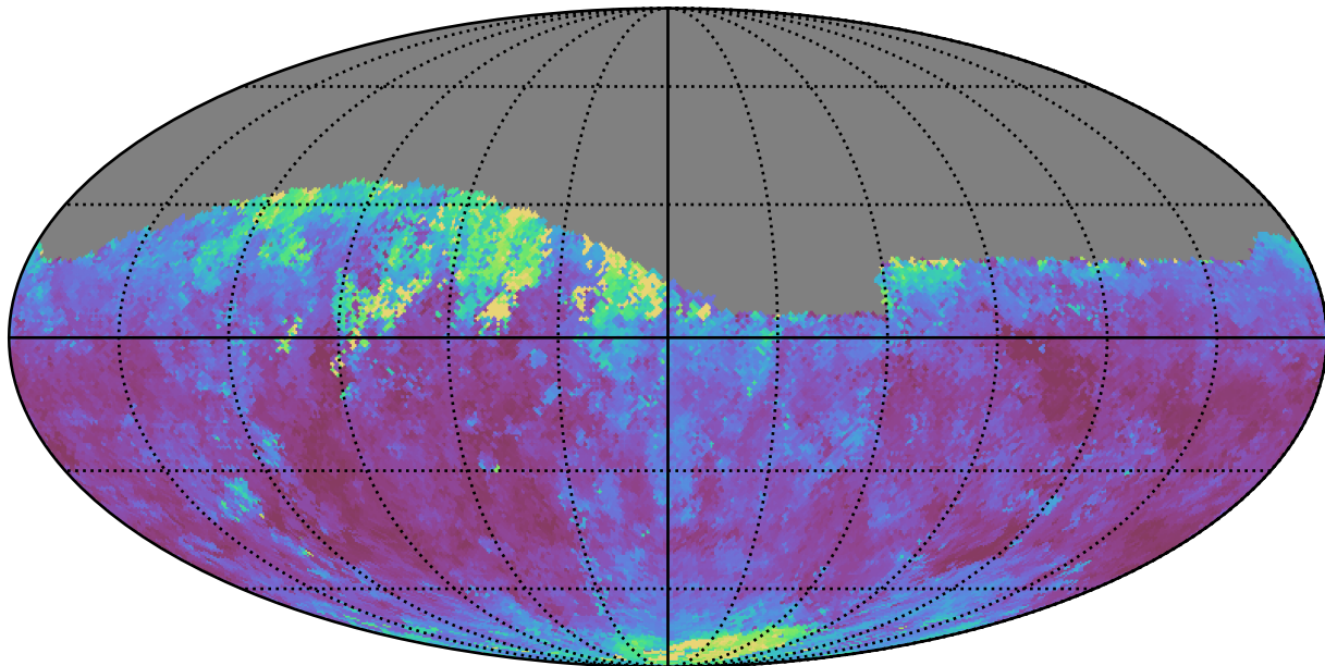
weather_cloudso36v3.4_10yrs Yr 1 r band: Median seeingEff
