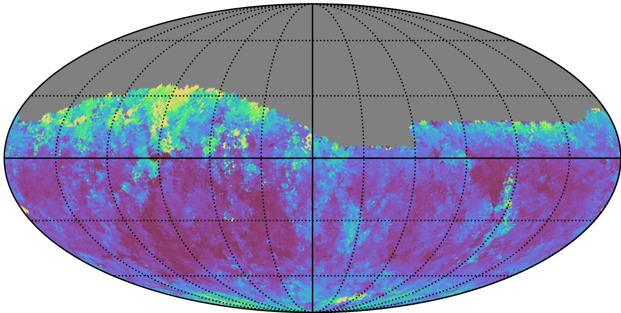
weather_cloudso36v3.4_10yrs Yr 1 i band: Median seeingEff
