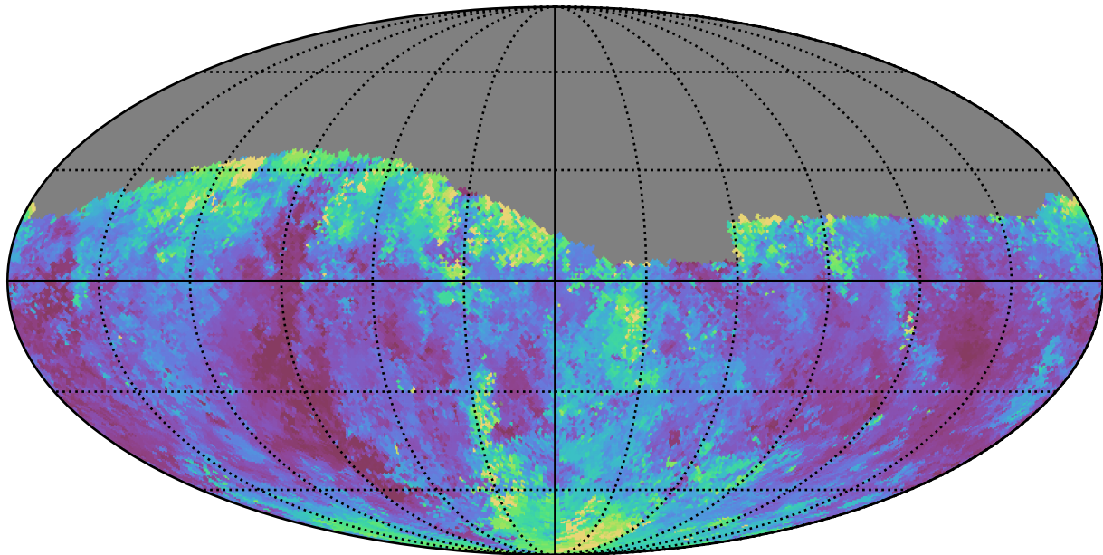
weather_cloudso36v3.4_10yrs Yr 1 g band: Median seeingEff
