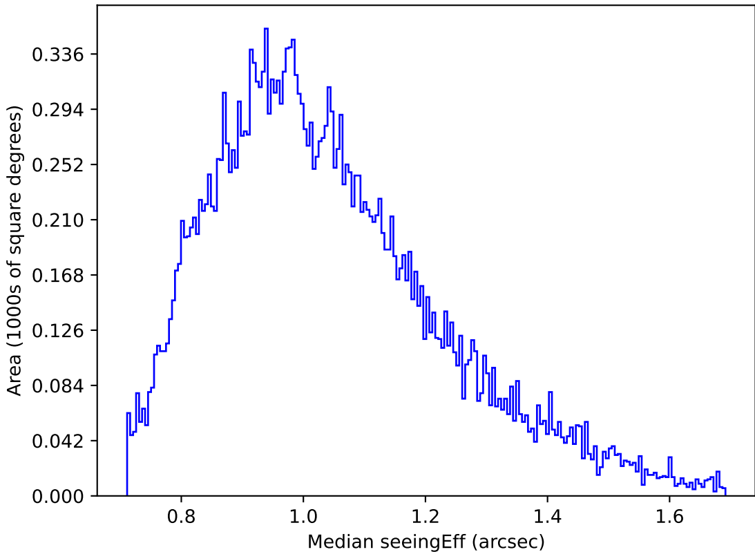
weather_cloudso36v3.4_10yrs Yr 1 g band: Median seeingEff
