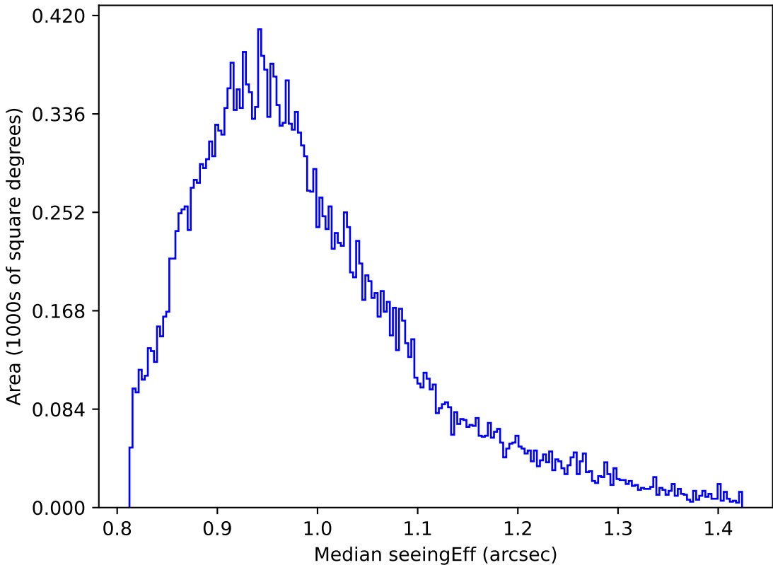
weather_cloudso36v3.4_10yrs Yr 1 all bands: Median seeingEff
