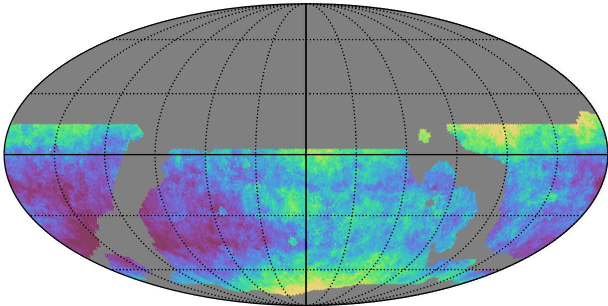
weather_cloudso36v3.4_10yrs WFD z band: Median seeingEff
