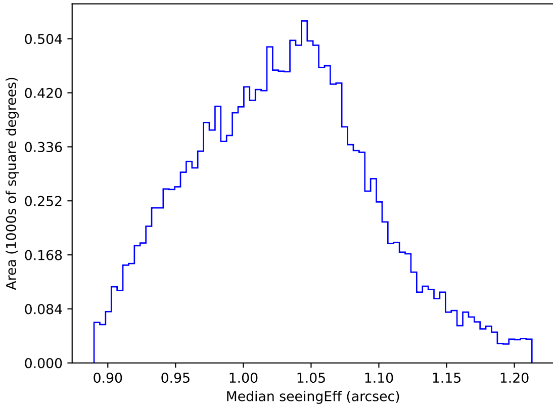
weather_cloudso36v3.4_10yrs WFD z band: Median seeingEff
