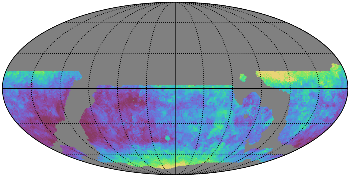
weather_cloudso36v3.4_10yrs WFD y band: Median seeingEff
