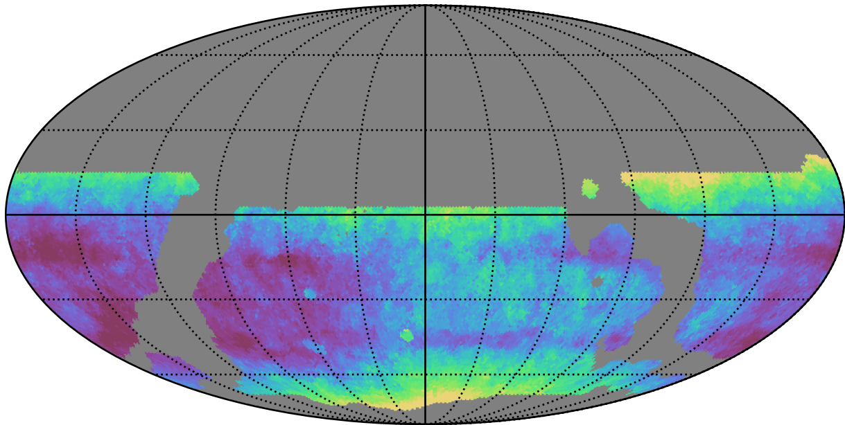
weather_cloudso36v3.4_10yrs WFD r band: Median seeingEff
