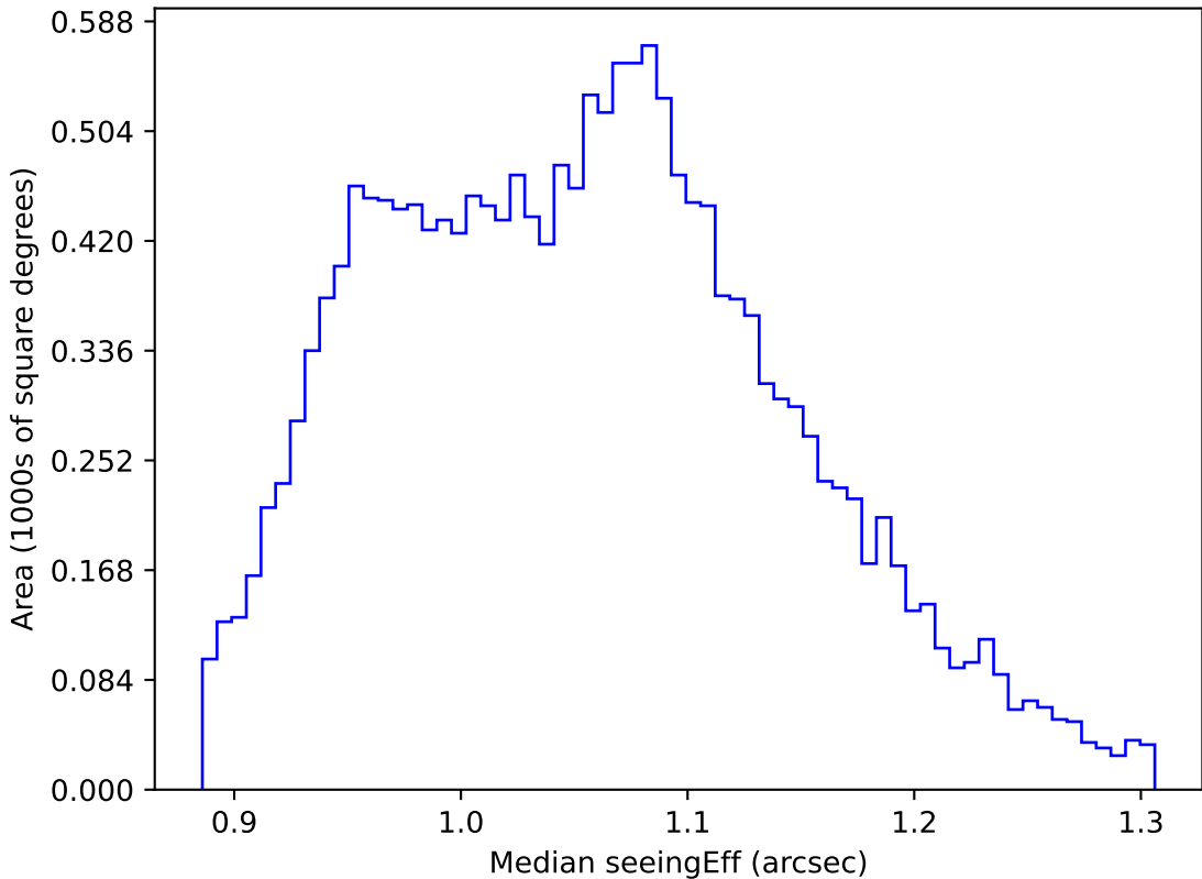
weather_cloudso36v3.4_10yrs WFD r band: Median seeingEff
