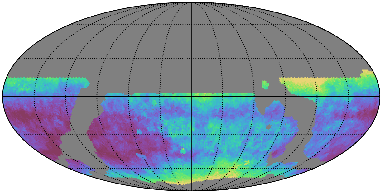
weather_cloudso36v3.4_10yrs WFD i band: Median seeingEff
