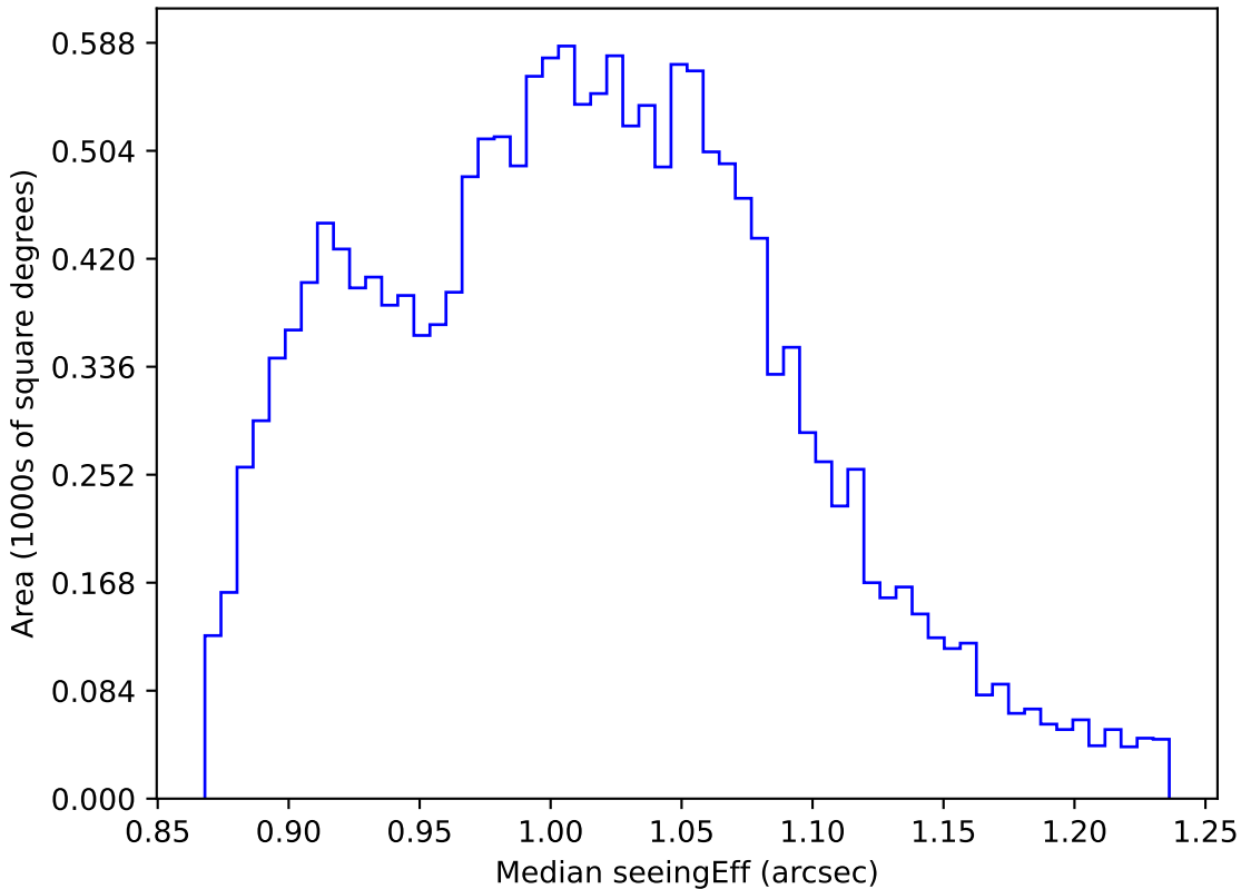
weather_cloudso36v3.4_10yrs WFD i band: Median seeingEff
