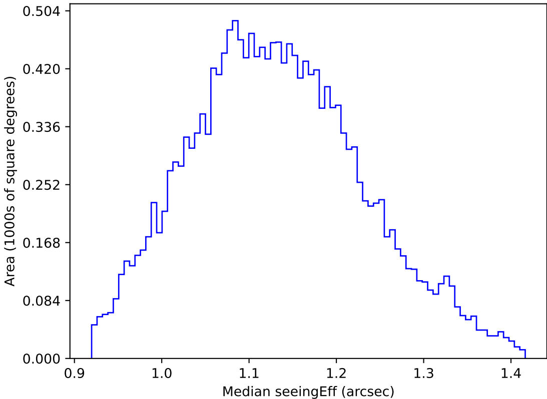
weather_cloudso36v3.4_10yrs WFD g band: Median seeingEff
