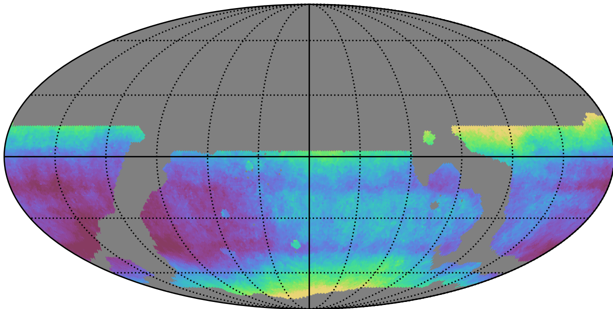
weather_cloudso36v3.4_10yrs WFD all bands: Median seeingEff
