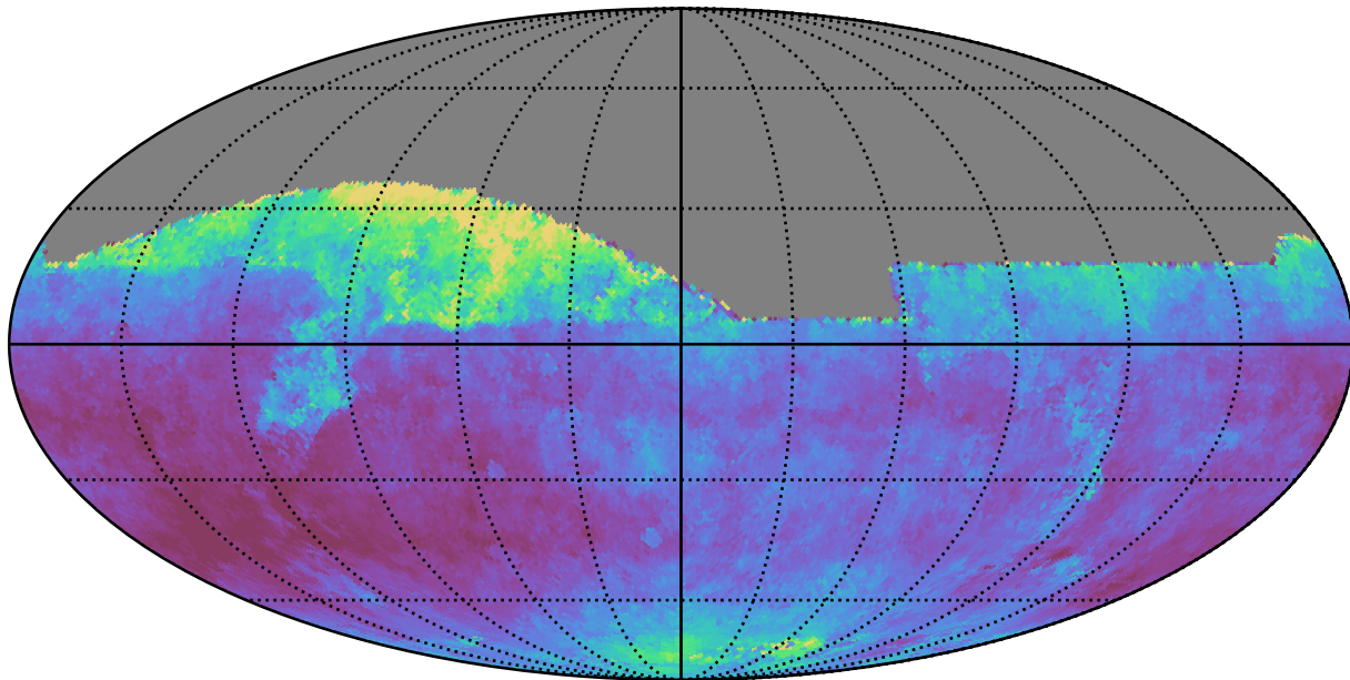
weather_cloudso36v3.4_10yrs All sky z band: Median seeingEff
