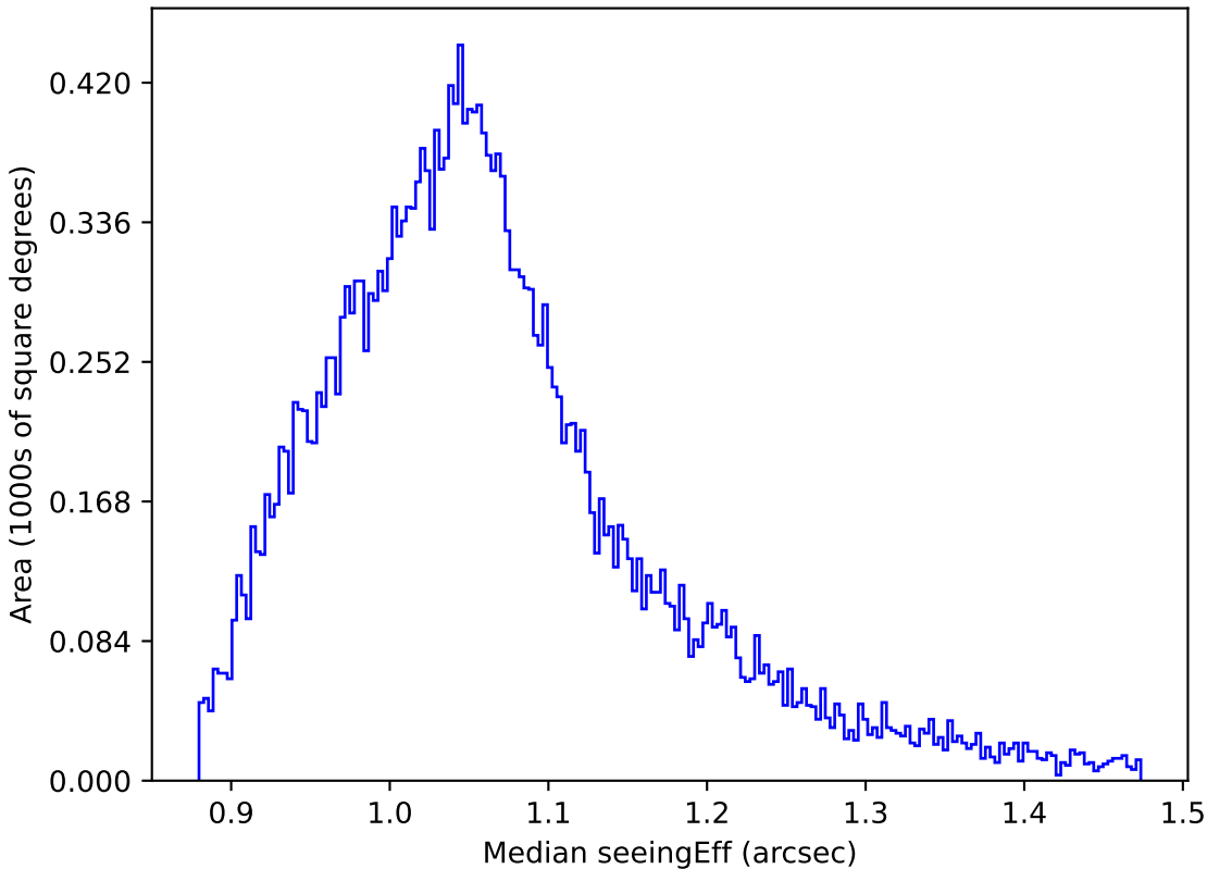
weather_cloudso36v3.4_10yrs All sky z band: Median seeingEff
