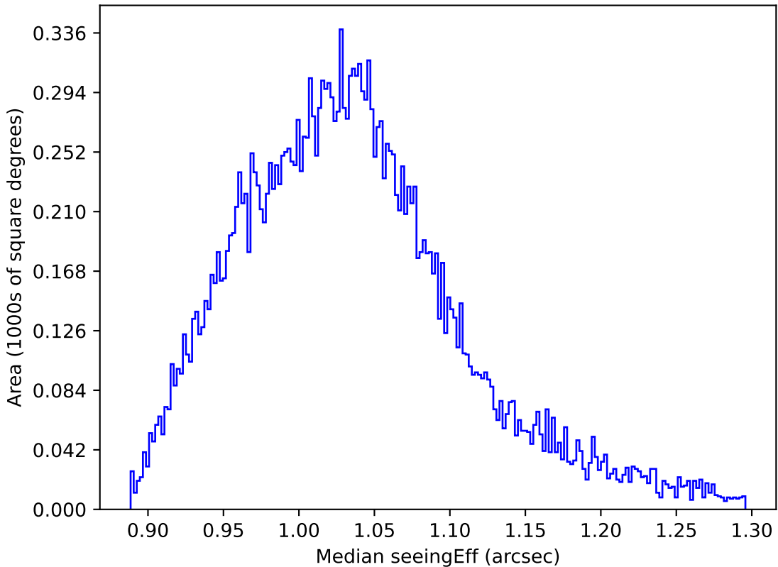
weather_cloudso36v3.4_10yrs All sky y band: Median seeingEff
