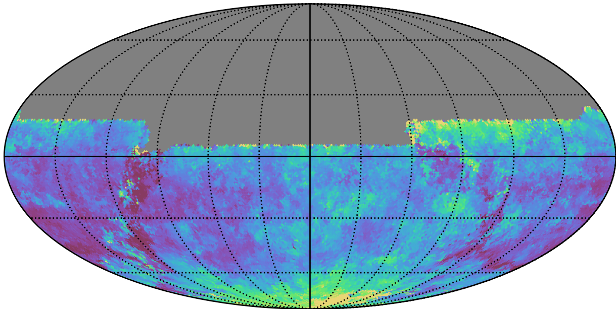
weather_cloudso36v3.4_10yrs All sky u band: Median seeingEff
