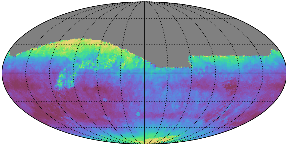
weather_cloudso36v3.4_10yrs All sky r band: Median seeingEff
