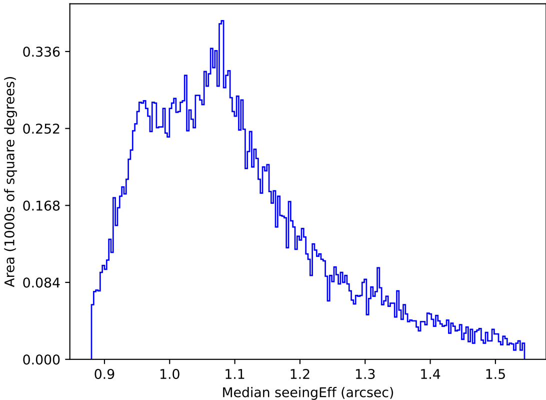
weather_cloudso36v3.4_10yrs All sky r band: Median seeingEff
