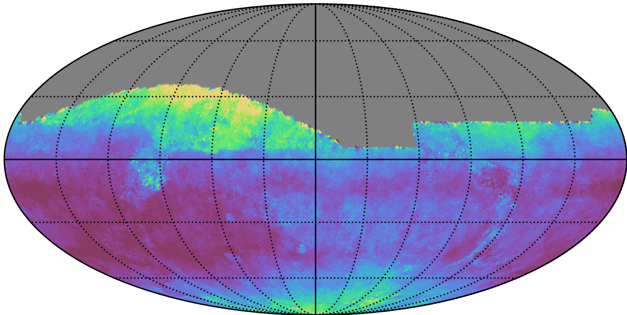
weather_cloudso36v3.4_10yrs All sky i band: Median seeingEff
