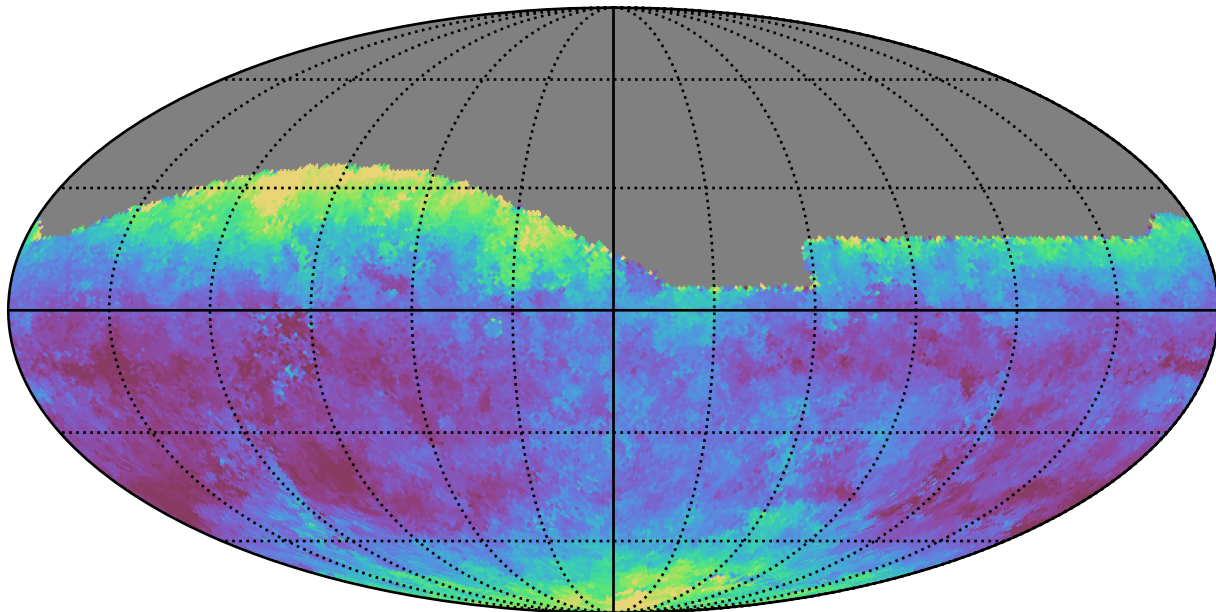
weather_cloudso36v3.4_10yrs All sky g band: Median seeingEff
