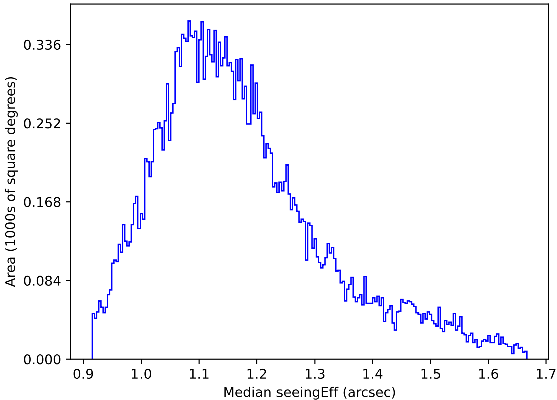
weather_cloudso36v3.4_10yrs All sky g band: Median seeingEff
