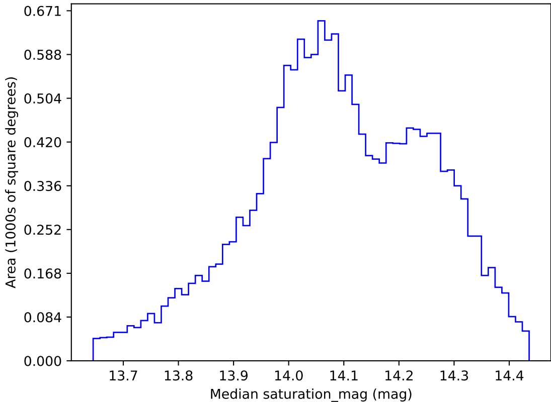
weather_cloudso36v3.4_10yrs WFD all bands: Median saturation_mag
