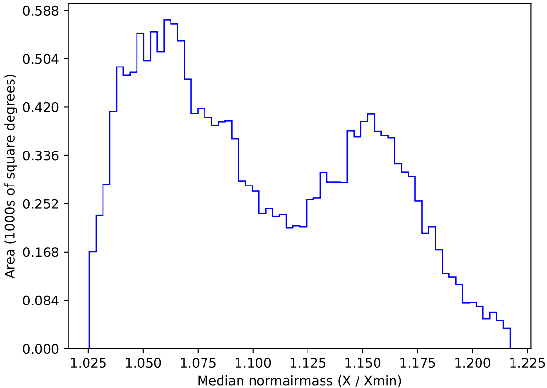
weather_cloudso36v3.4_10yrs WFD z band: Median normairmass
