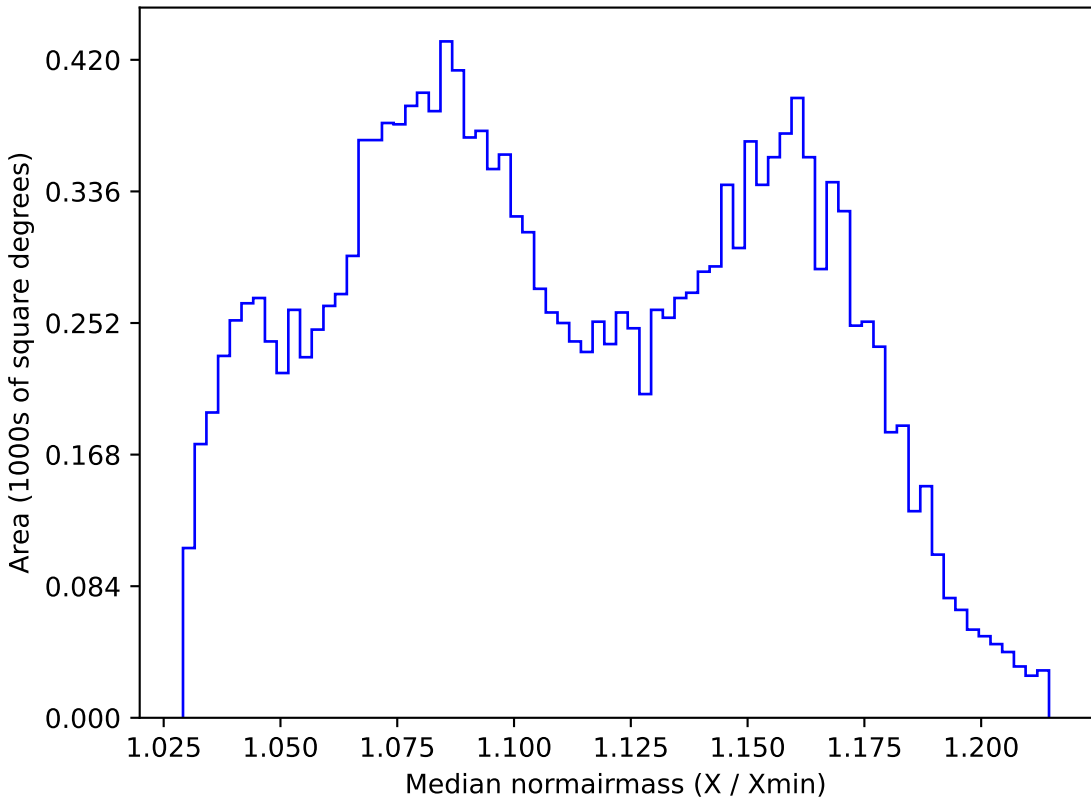
weather_cloudso36v3.4_10yrs WFD y band: Median normairmass
