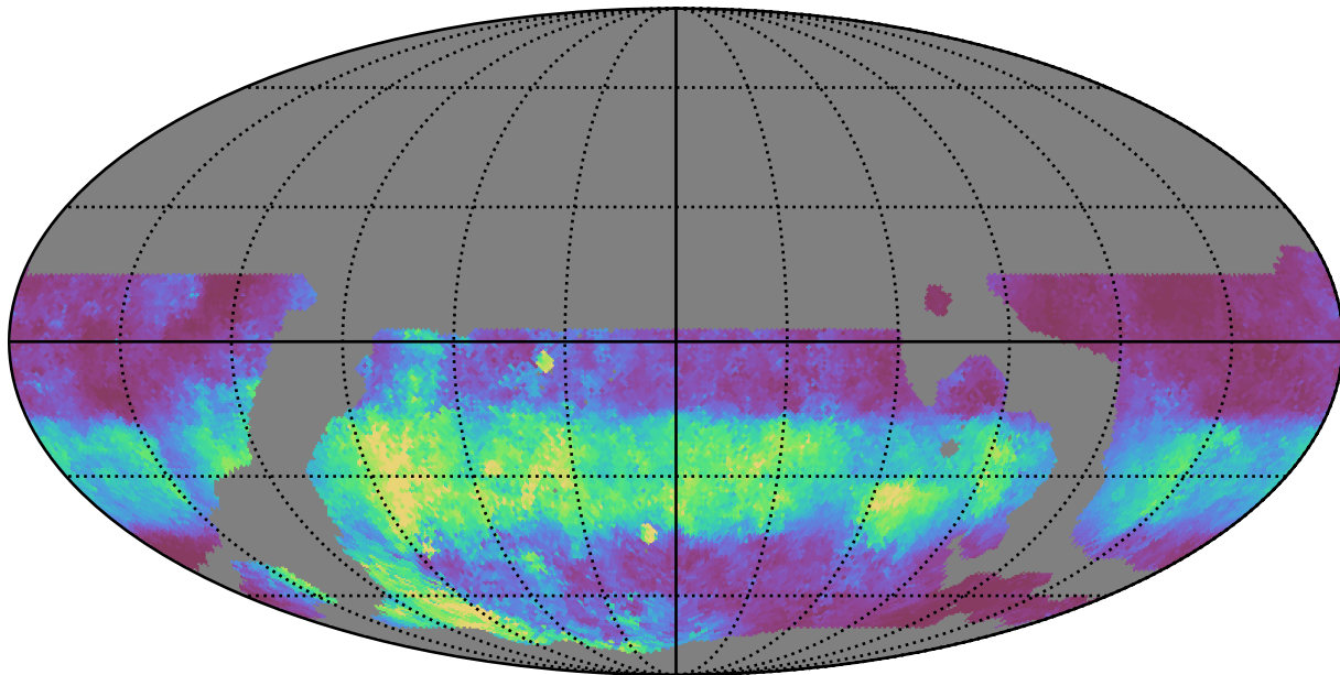
weather_cloudso36v3.4_10yrs WFD u band: Median normairmass
