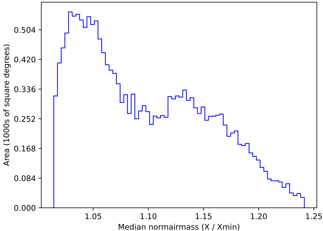
weather_cloudso36v3.4_10yrs WFD u band: Median normairmass
