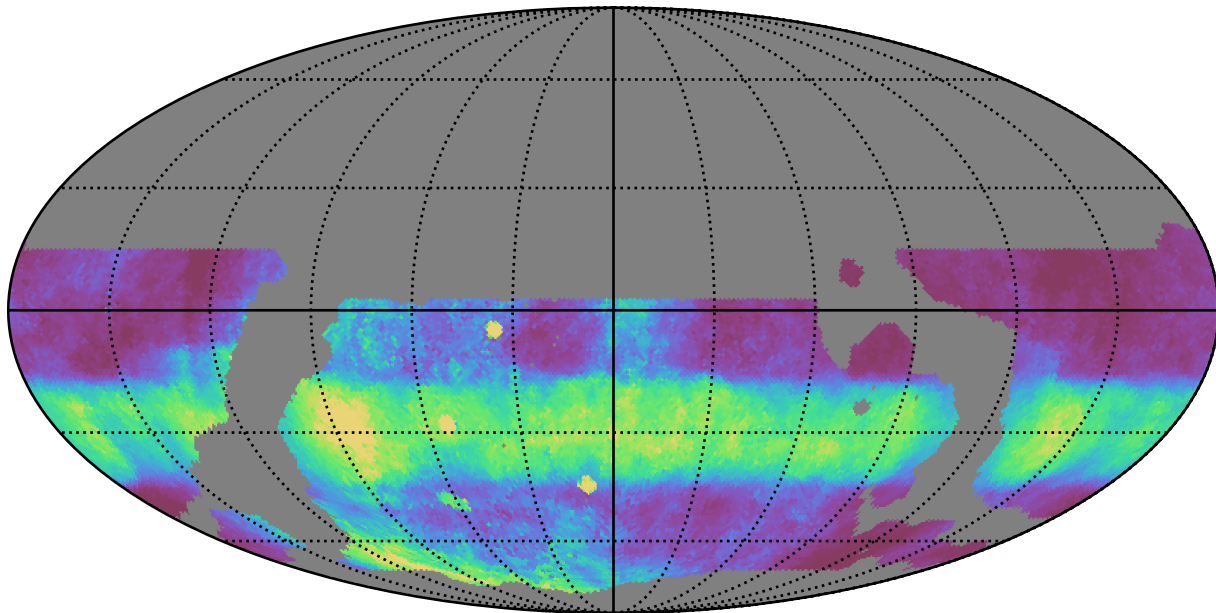
weather_cloudso36v3.4_10yrs WFD r band: Median normairmass
