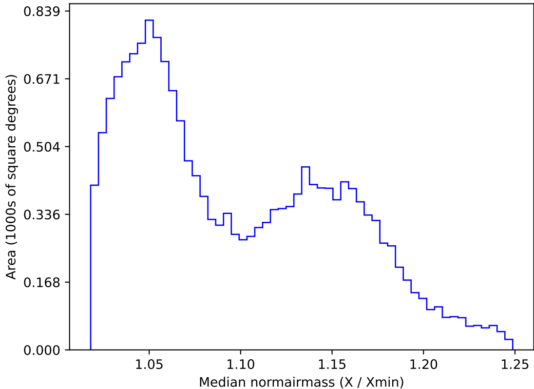
weather_cloudso36v3.4_10yrs WFD g band: Median normairmass
