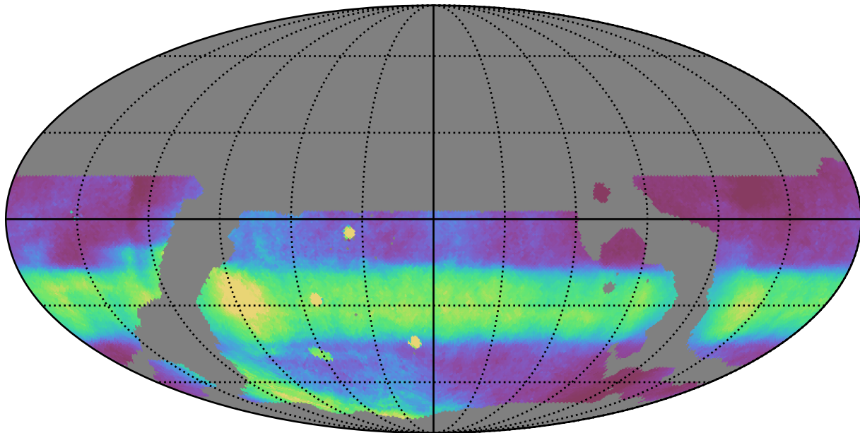
weather_cloudso36v3.4_10yrs WFD all bands: Median normairmass
