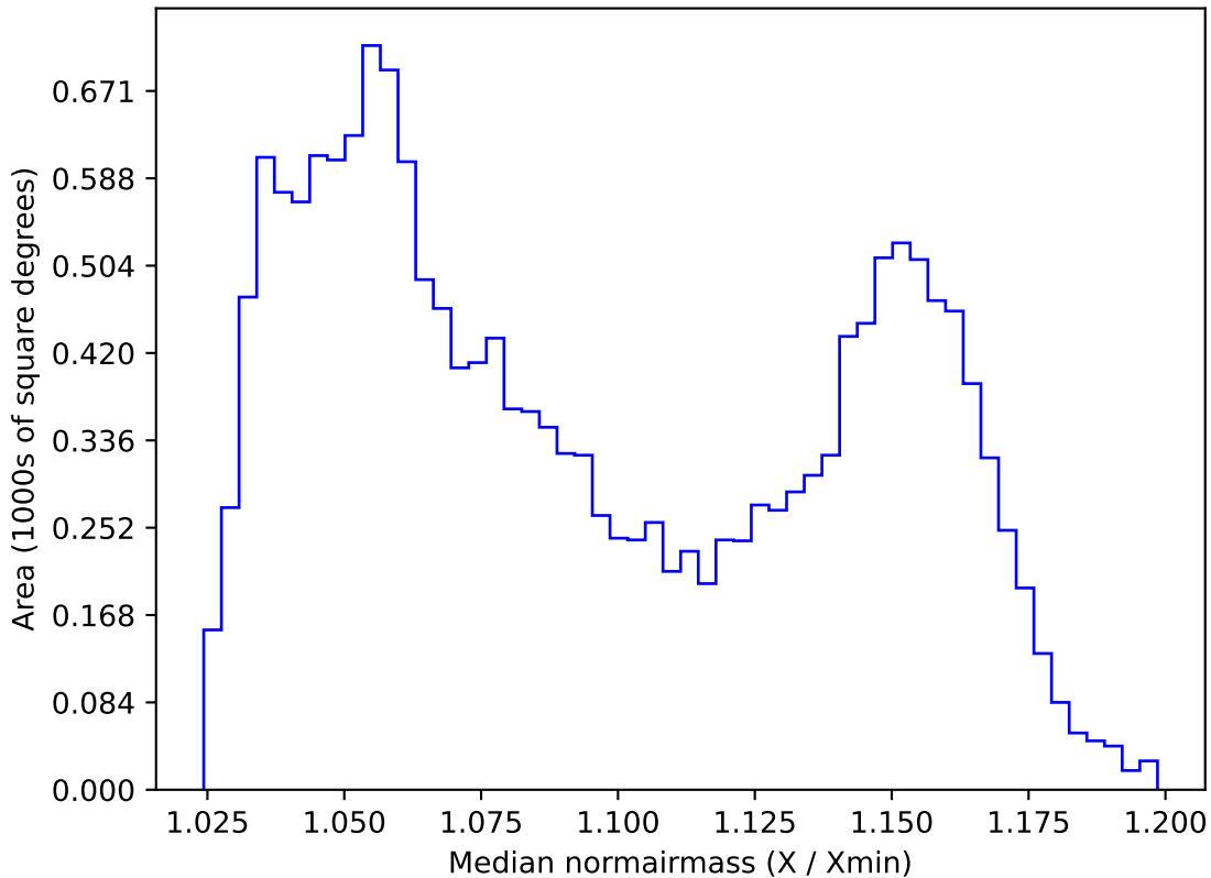
weather_cloudso36v3.4_10yrs WFD all bands: Median normairmass
