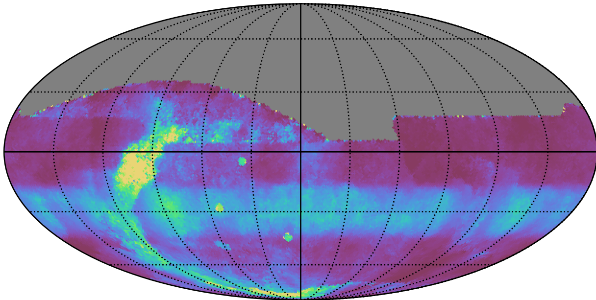
weather_cloudso36v3.4_10yrs All sky r band: Median normairmass
