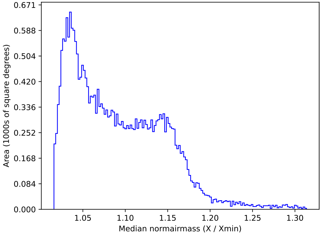
weather_cloudso36v3.4_10yrs All sky r band: Median normairmass
