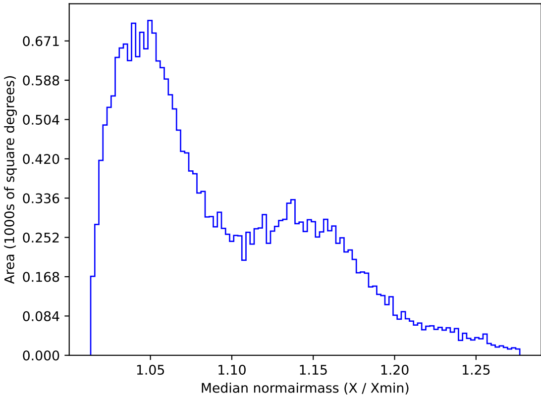
weather_cloudso36v3.4_10yrs All sky g band: Median normairmass
