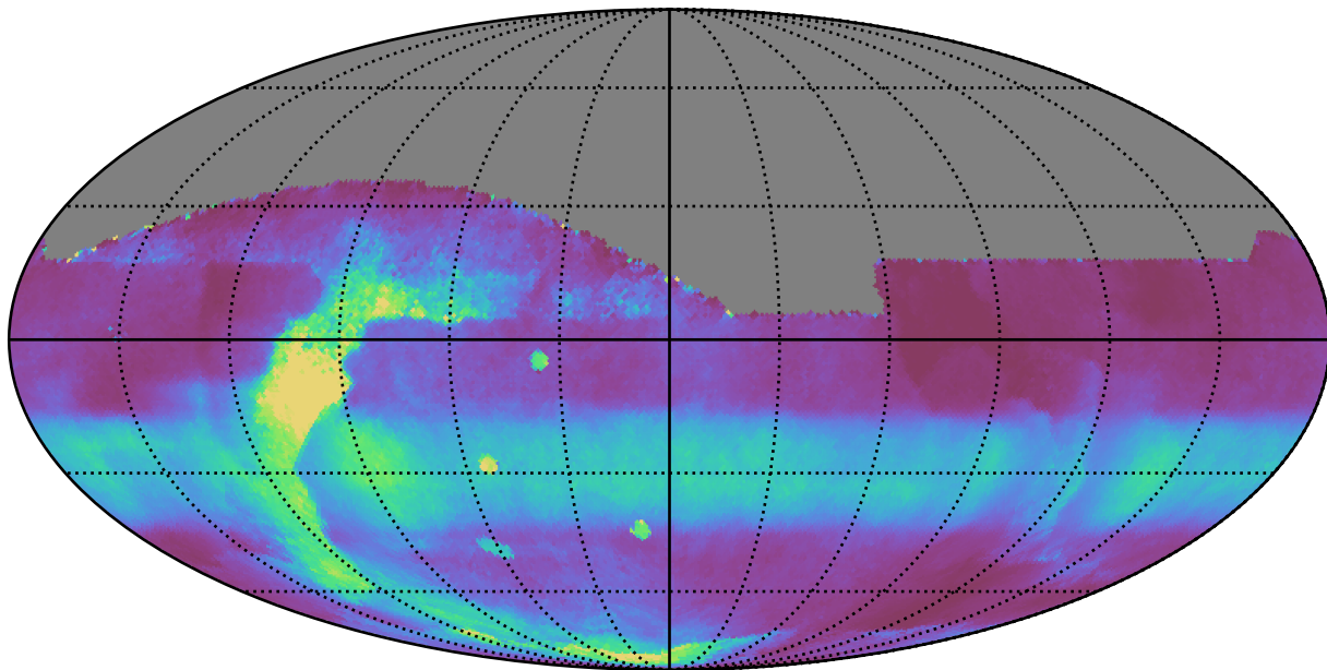
weather_cloudso36v3.4_10yrs All sky all bands: Median normairmass
