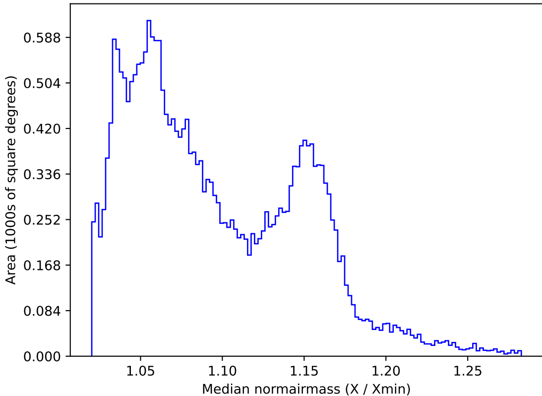
weather_cloudso36v3.4_10yrs All sky all bands: Median normairmass
