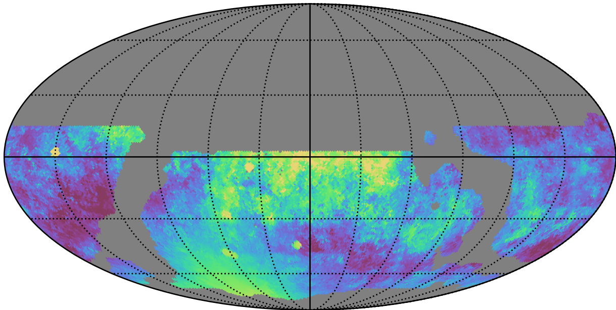
weather_cloudso36v3.4_10yrs WFD z band: Median moonDistance
