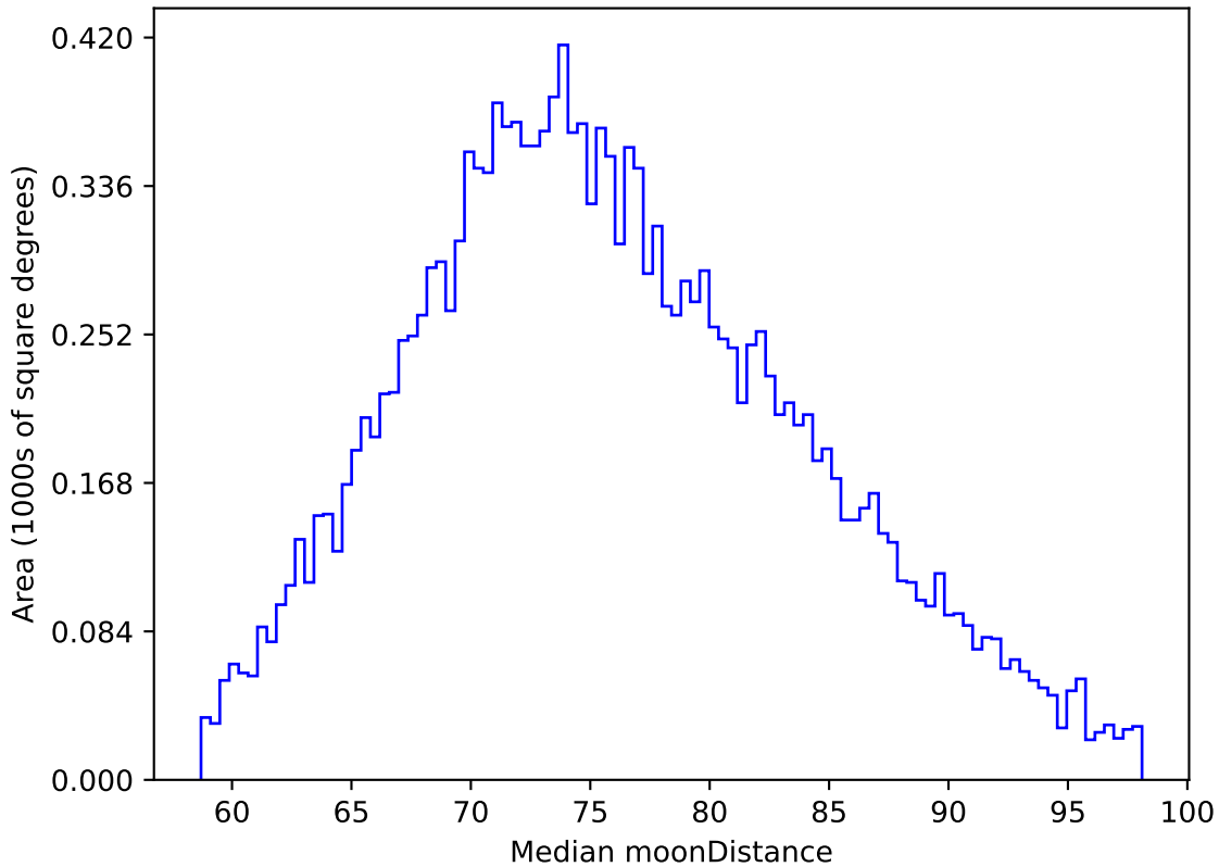
weather_cloudso36v3.4_10yrs WFD z band: Median moonDistance
