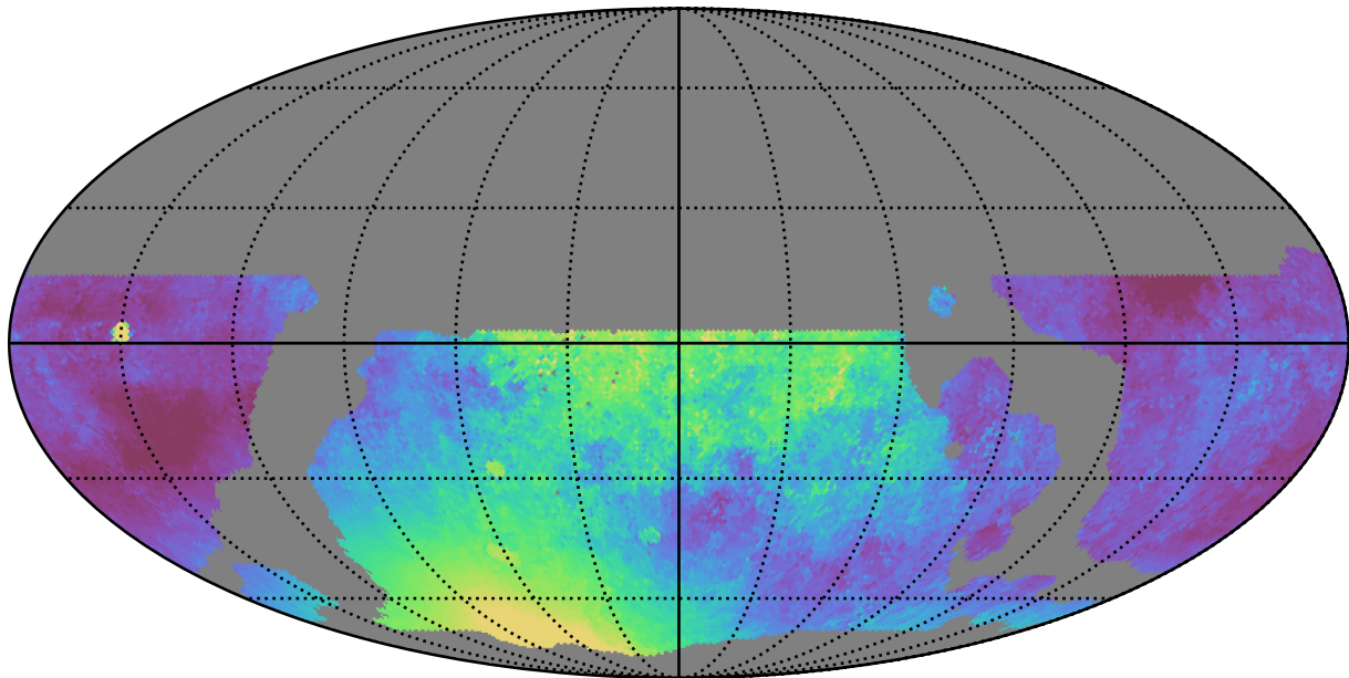
weather_cloudso36v3.4_10yrs WFD y band: Median moonDistance
