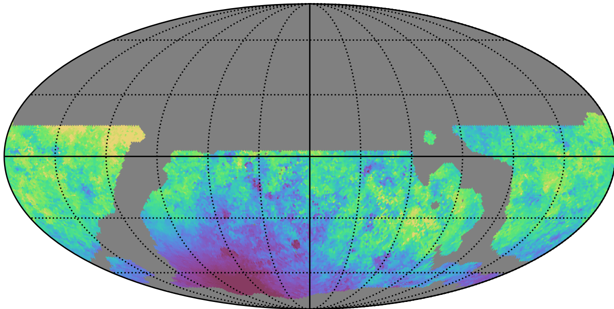
weather_cloudso36v3.4_10yrs WFD r band: Median moonDistance
